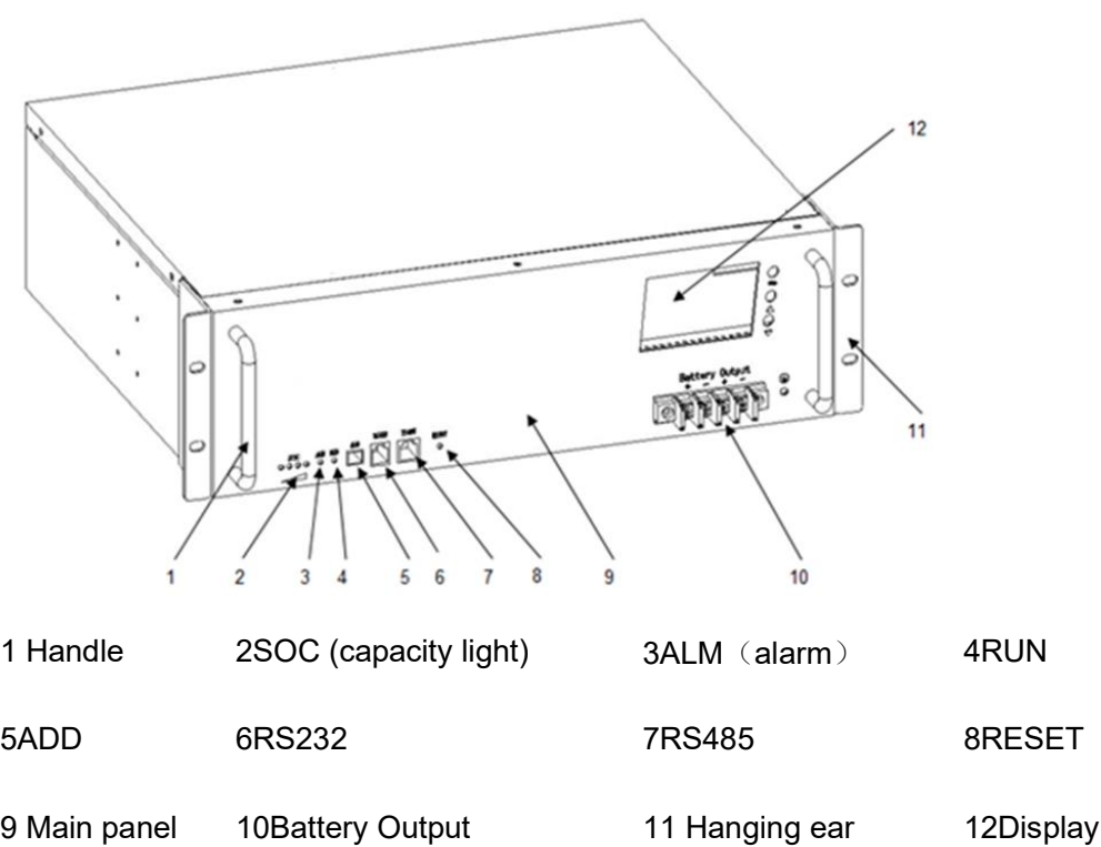
Figure2-1 Product structure
